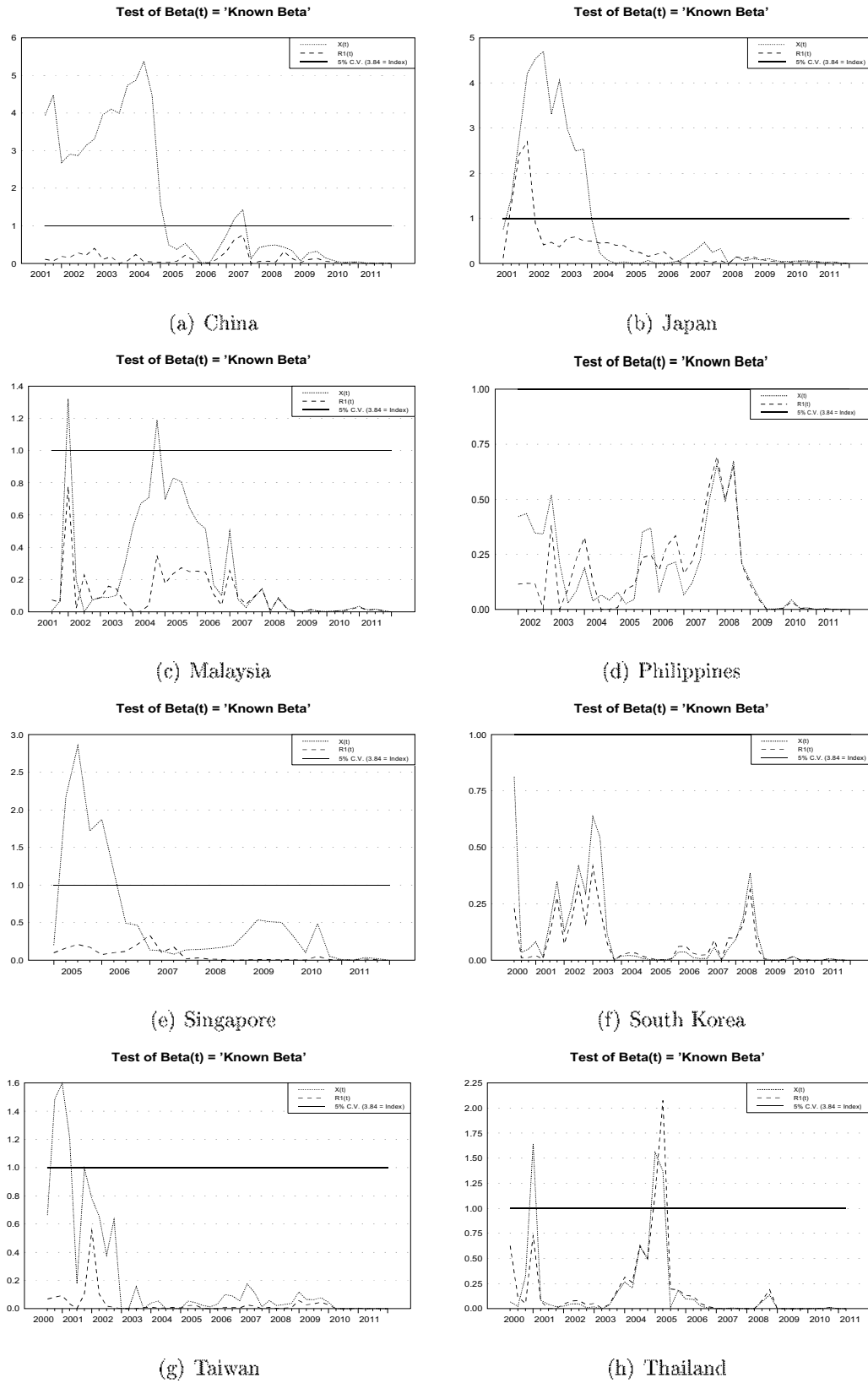
Figure 2: Test for \beta stability
