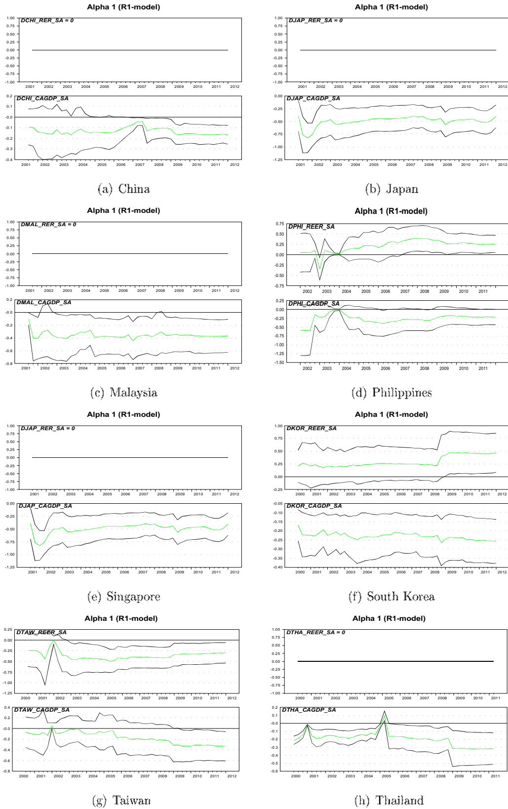
Figure 3: Test for \alpha stability
